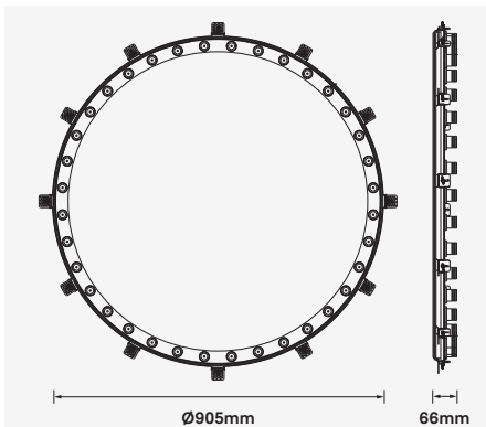
Ceiling cut-out Ø915mm / 9-25mm ceiling thickness
