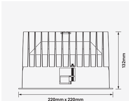
Ceiling cut-out 200mm x 200mm / 6-25mm ceiling thickness
